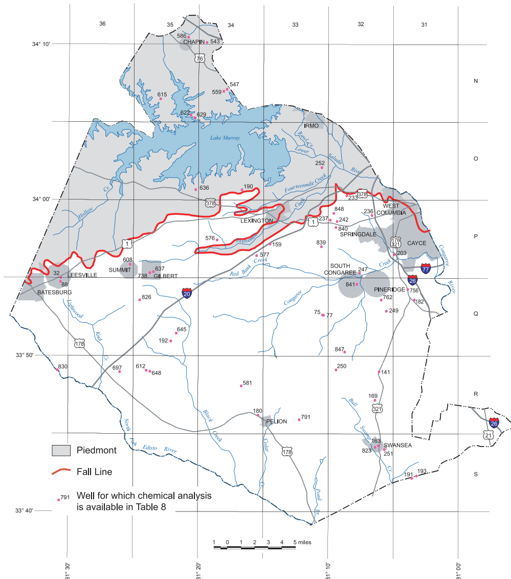
Figure 16. Locations of wells for which chemical analyses appear in Table 8.
