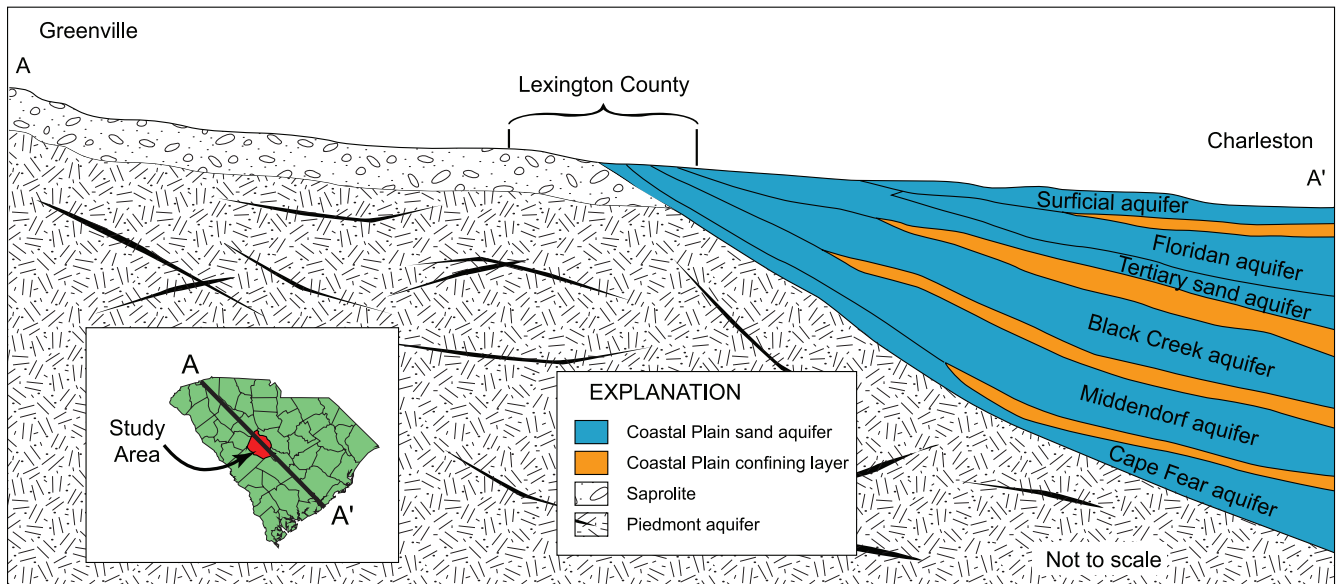
Figure 10. Generalized subsurface geology of Lexington County (modified from Aucott and others, (1987).
