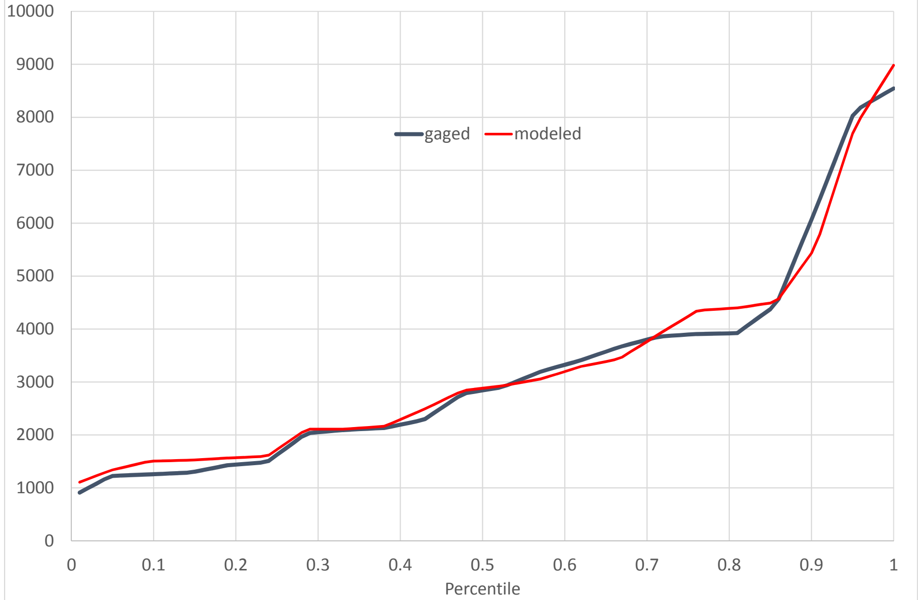
BRD22 (021564493) BROAD RIVER BELOW NEAL SHOALS RES. NR CARLISLE, SC Monthly Flow Percentiles (CFS)
