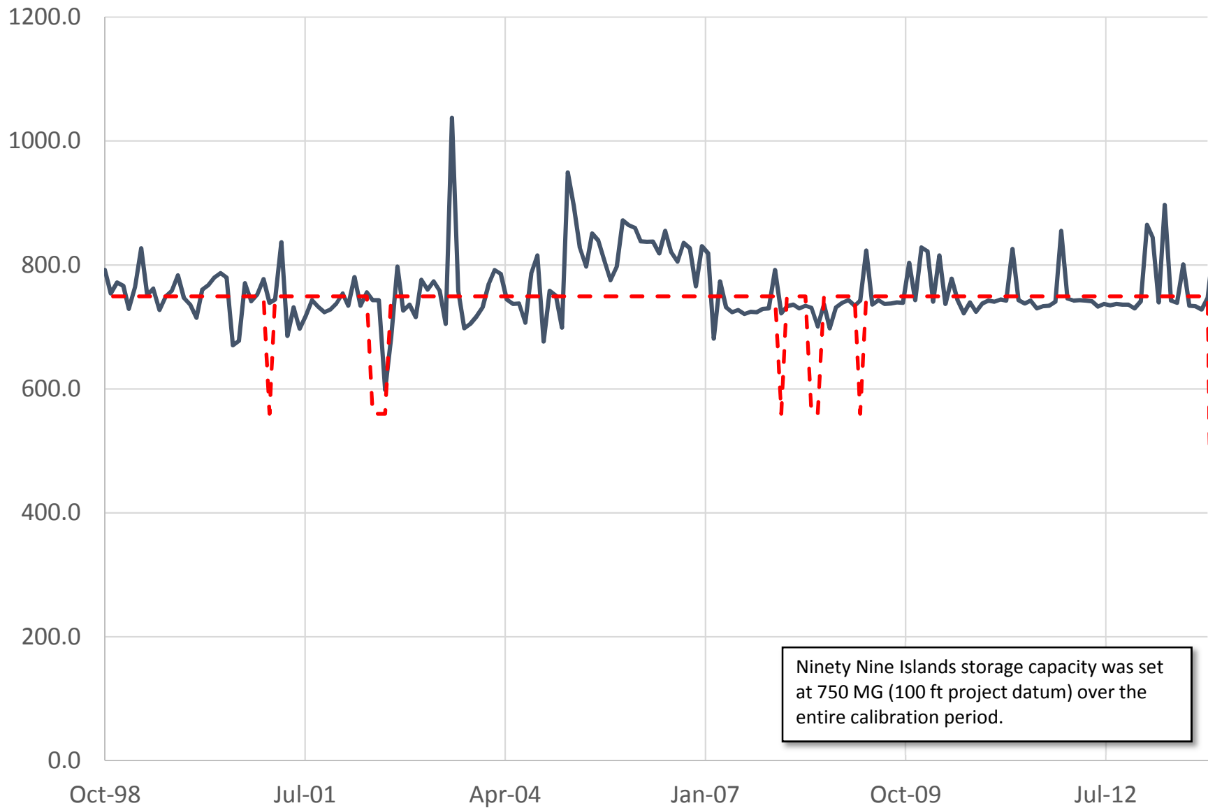
Ninety Nine Islands Storage (MG)
