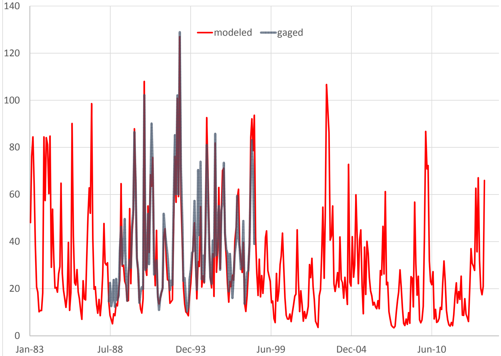
BRD40 (02159810) FAIRFOREST CREEK BELOW SPARTANBURG, S.C. (CFS)
