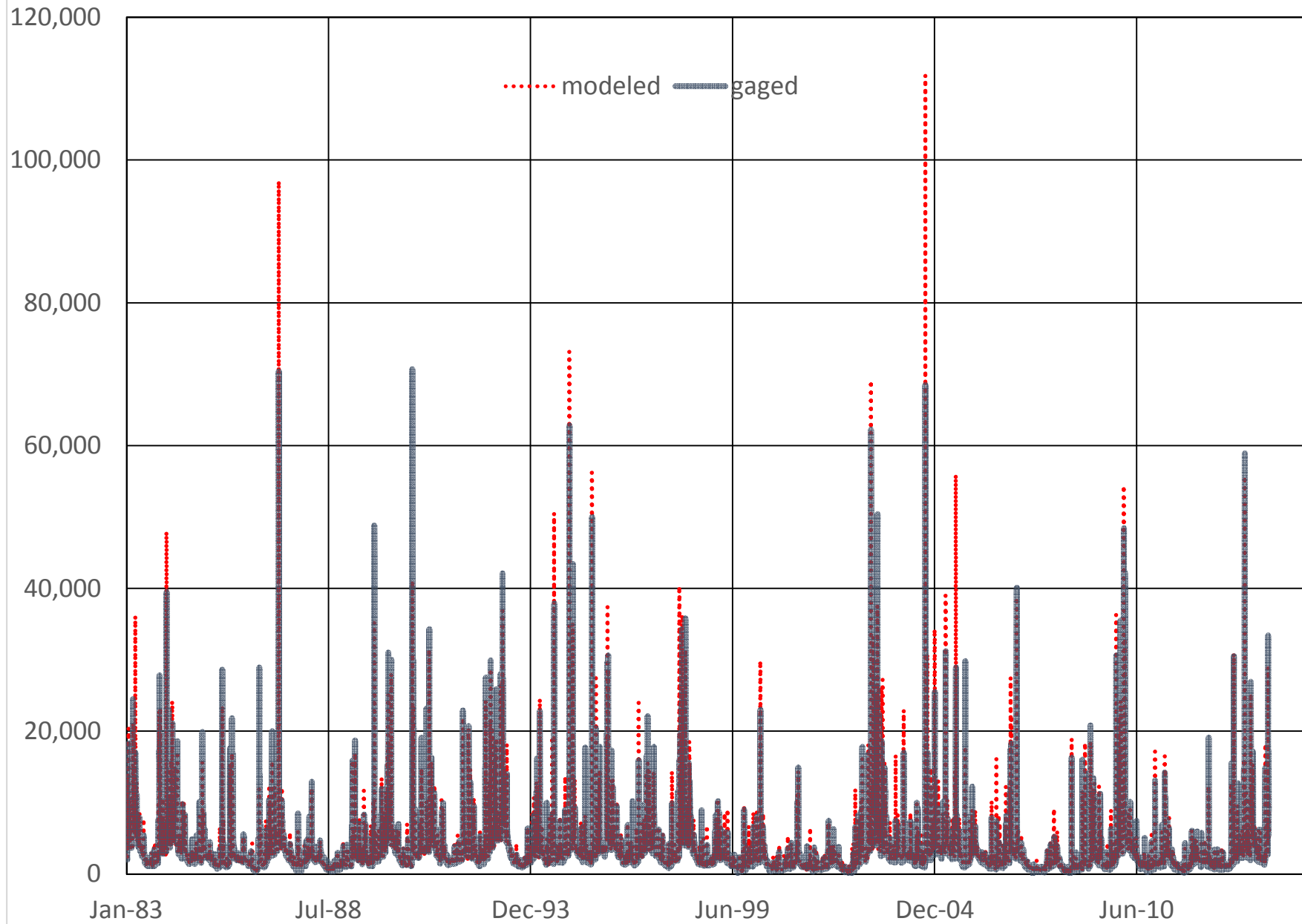
BRD24 (02156500) BROAD RIVER NEAR CARLISLE, SC (CFS)
