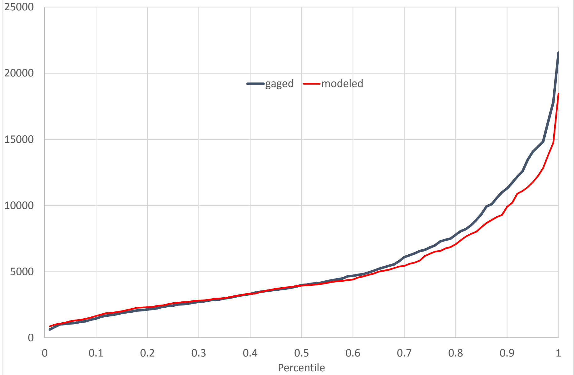
BRD54 (02161000) BROAD RIVER AT ALSTON, SC Monthly Flow Percentiles (CFS)
