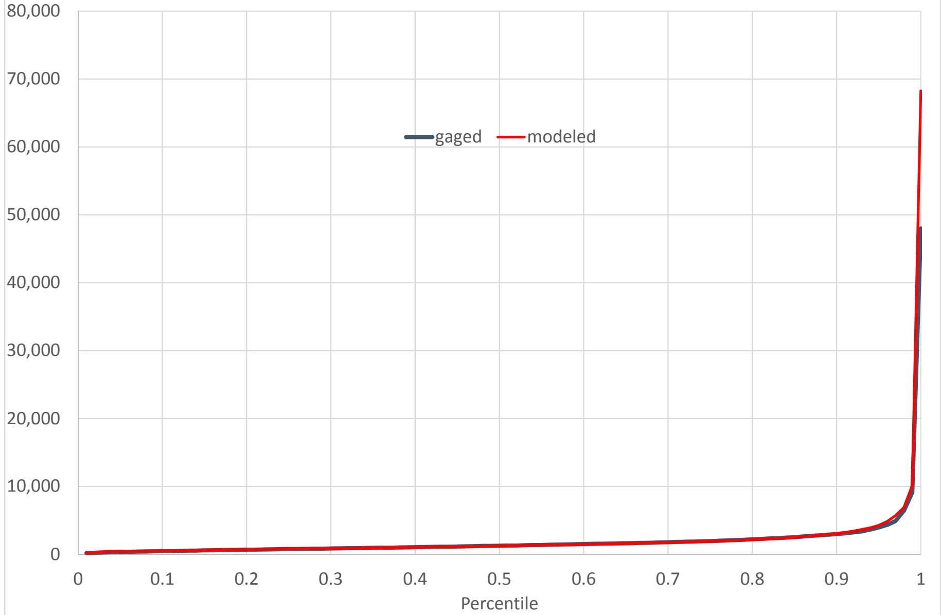
BRD01 (02153200) BROAD RIVER NEAR BLACKSBURG, SC Daily Flow Percentiles (CFS)
