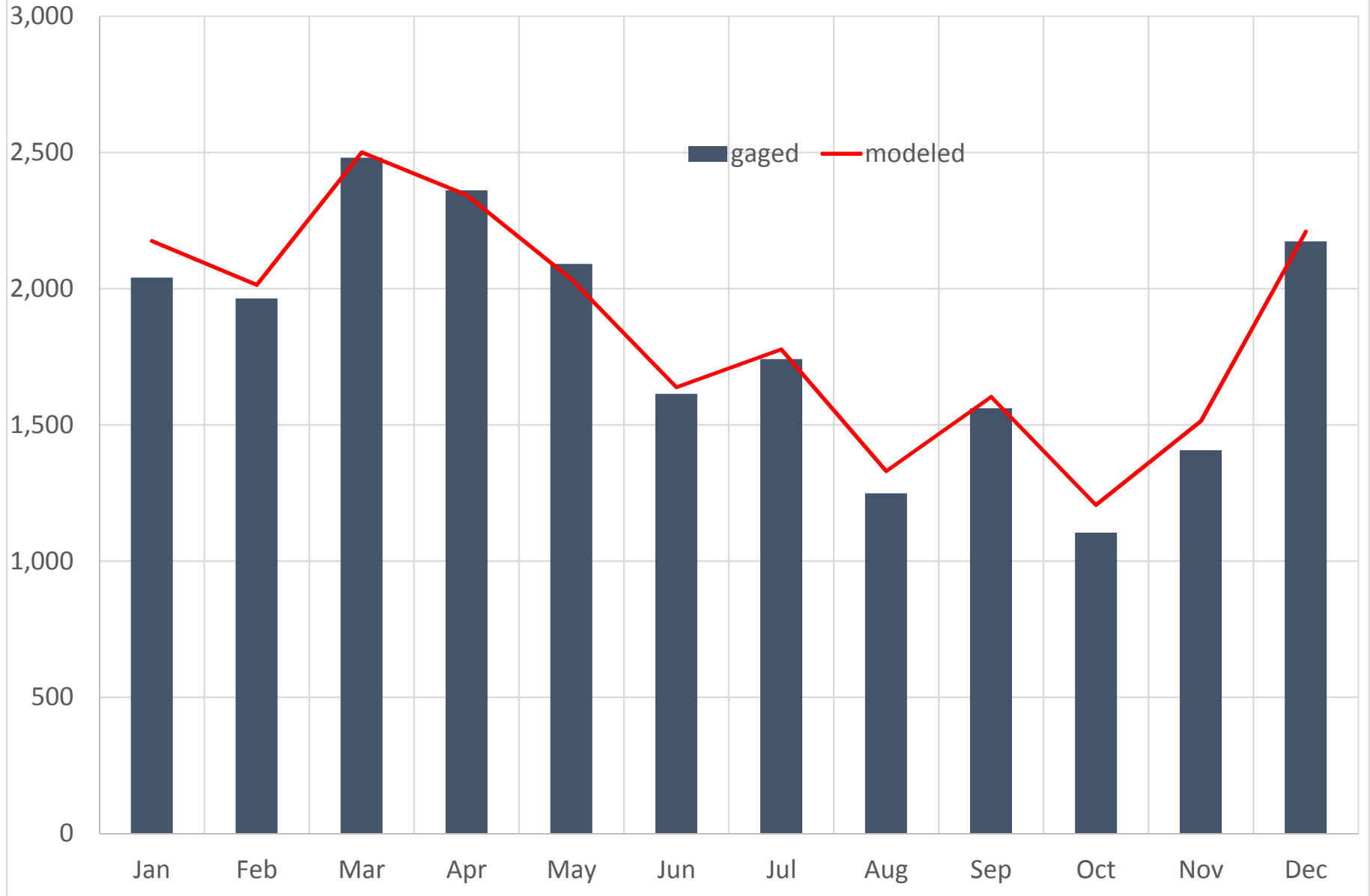
BRD03 (02153551) BROAD RIVER BELOW NINETYNINE ISLAND RESERVOIR, SC Monthly Mean Flow (CFS)
