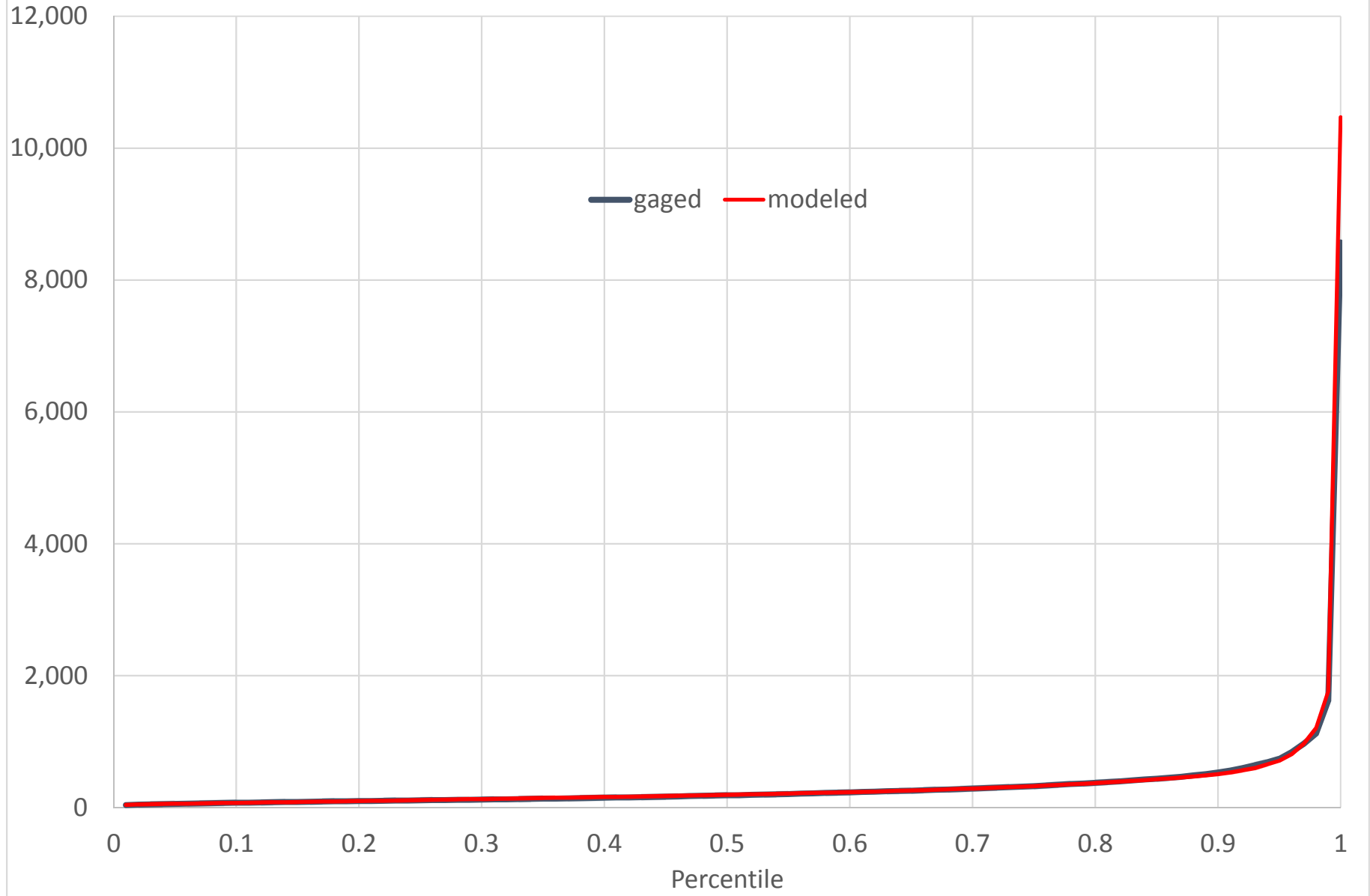
BRD12 (02155500) PACOLET RIVER NEAR FINGERVILLE, SC Daily Flow Percentiles (CFS)
