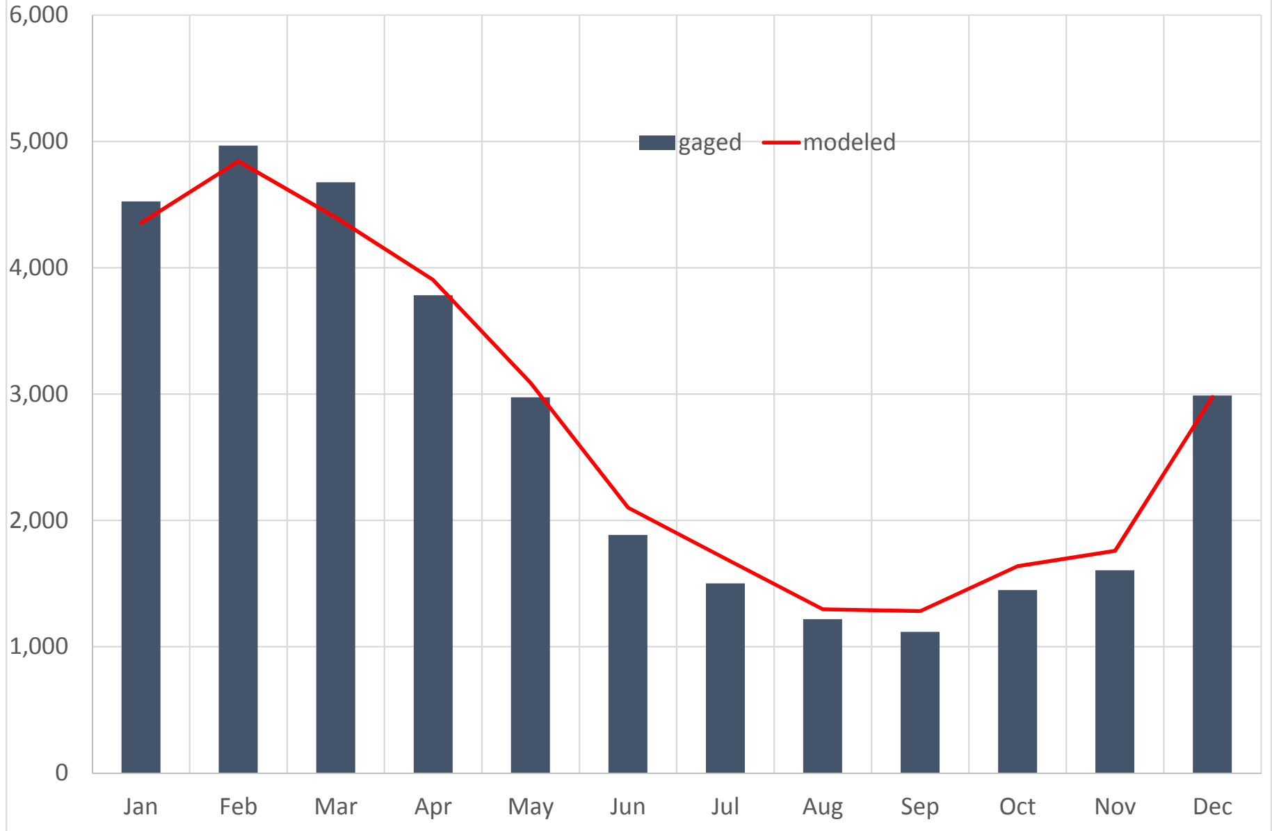
BRD21 (02156409) BROAD RIVER NEAR LOCKHART, SC Monthly Mean Flow (CFS)
