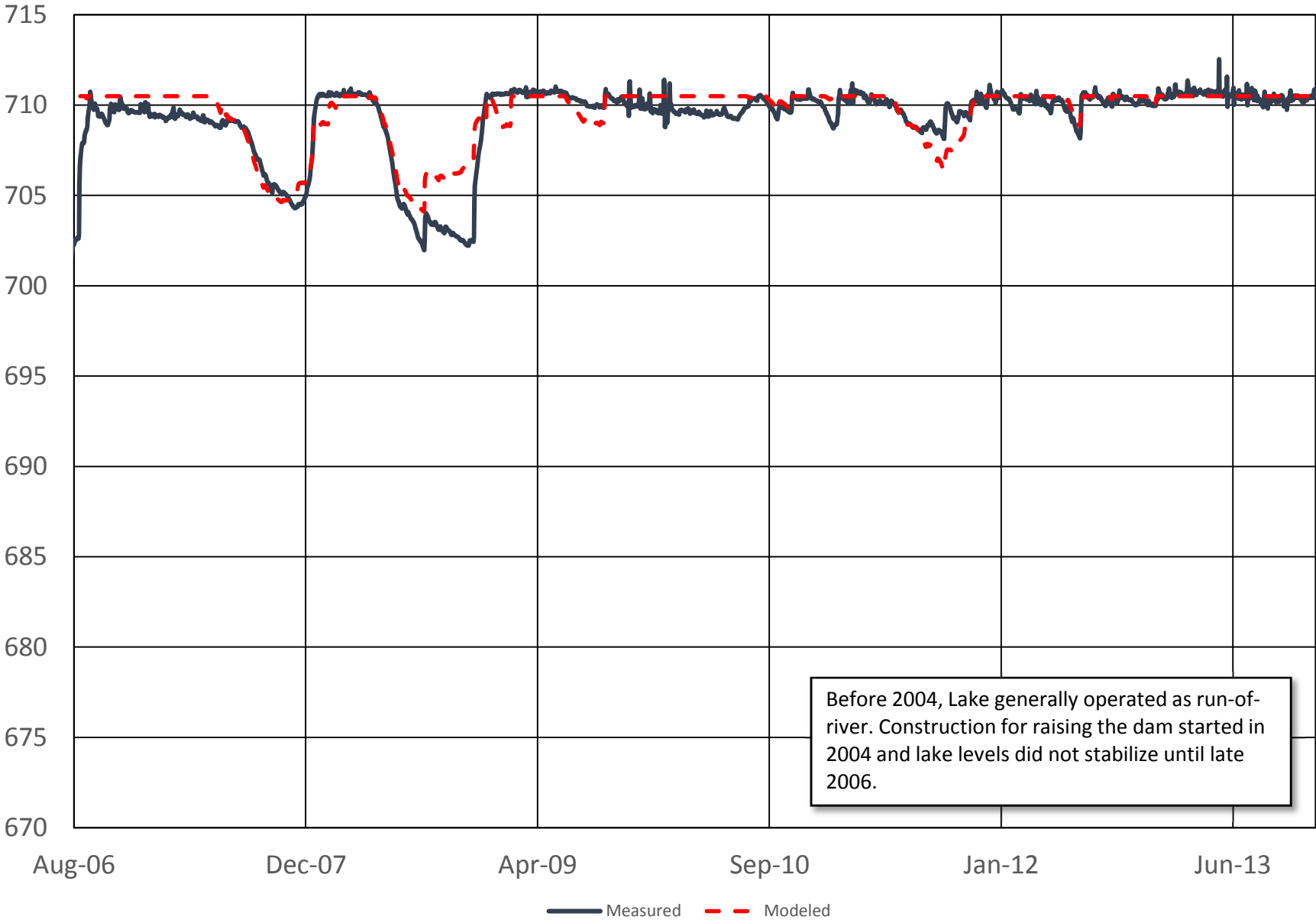
Lake Blalock Elevations (ft)
