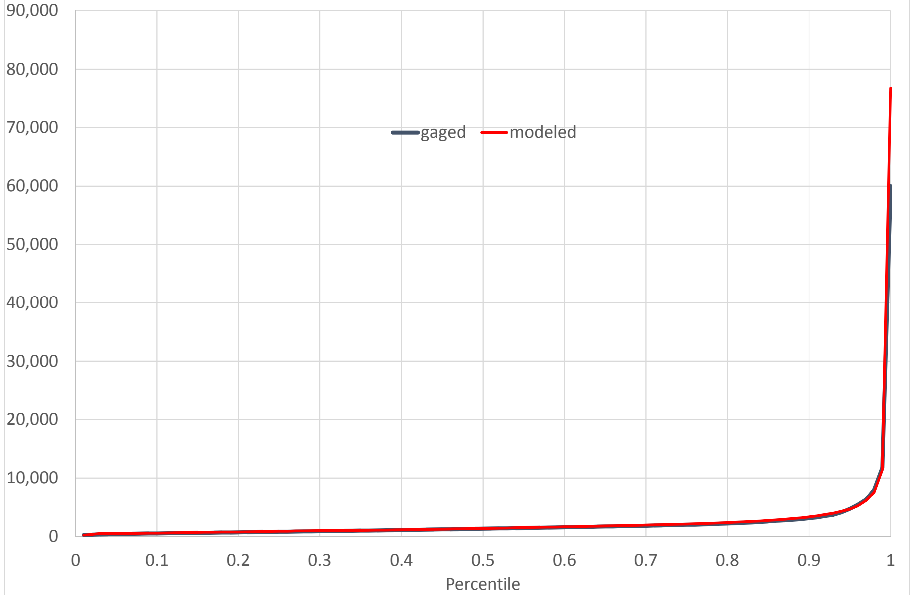
BRD03 (02153551) BROAD RIVER BELOW NINETYNINE ISLAND RESERVOIR, SC Daily Flow Percentiles (CFS)
