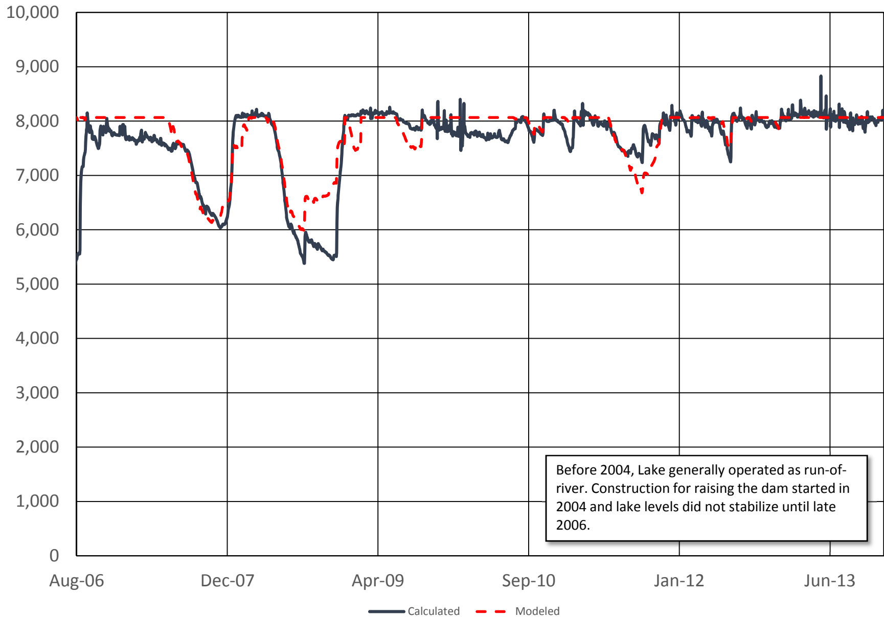
Lake Blalock Storage (MG)
