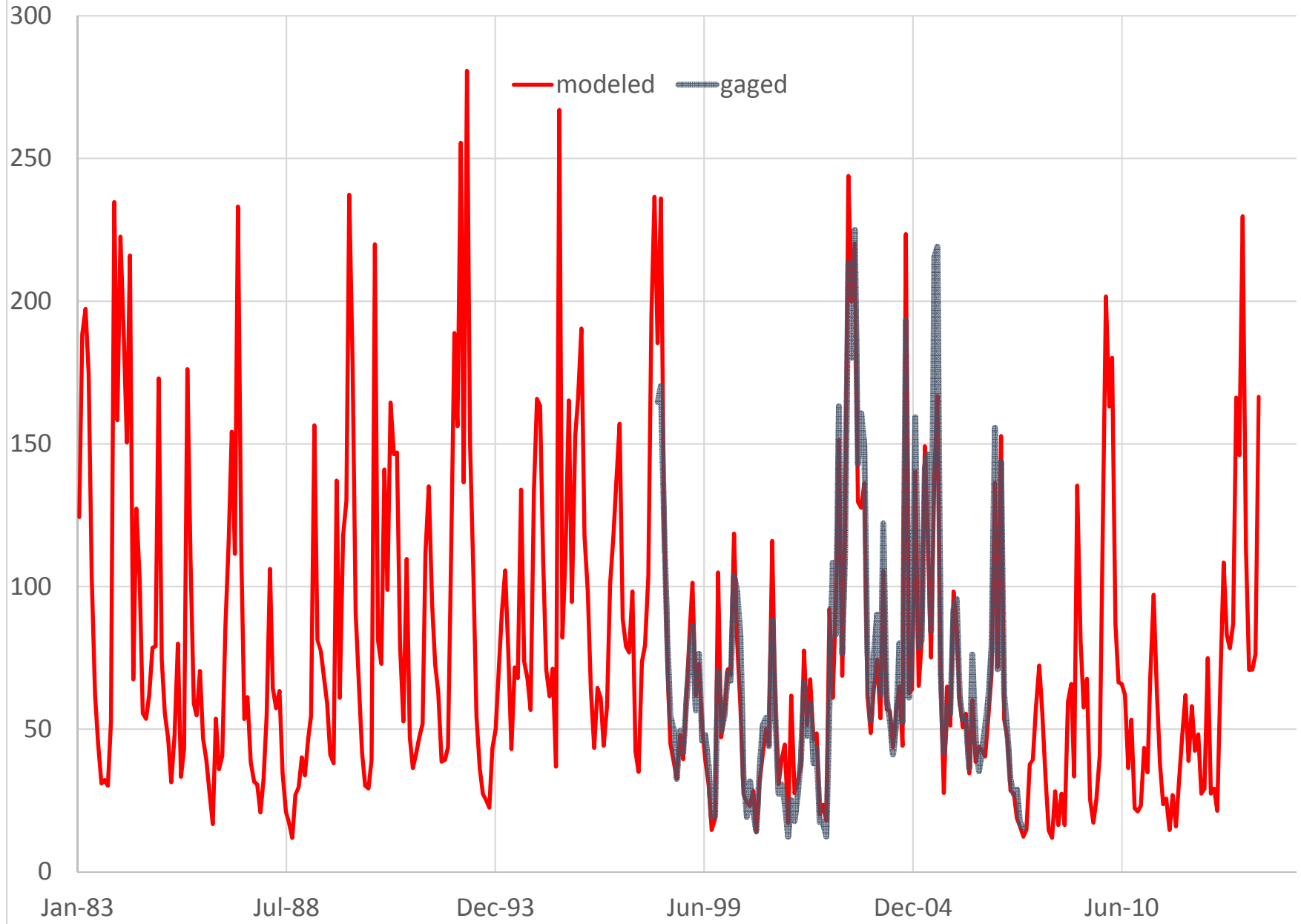
BRD43 (02160200) ENOREE RIVER AT TAYLORS, SC (CFS)
