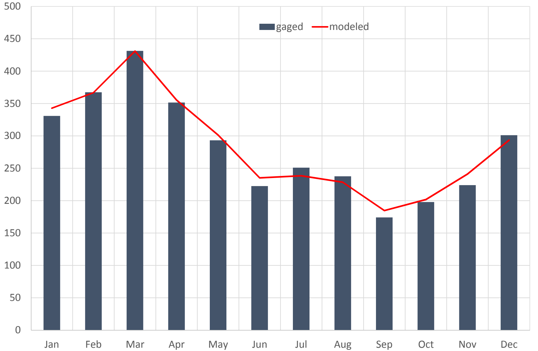
BRD12 (02155500) PACOLET RIVER NEAR FINGERVILLE, SC Monthly Mean Flow (CFS)
