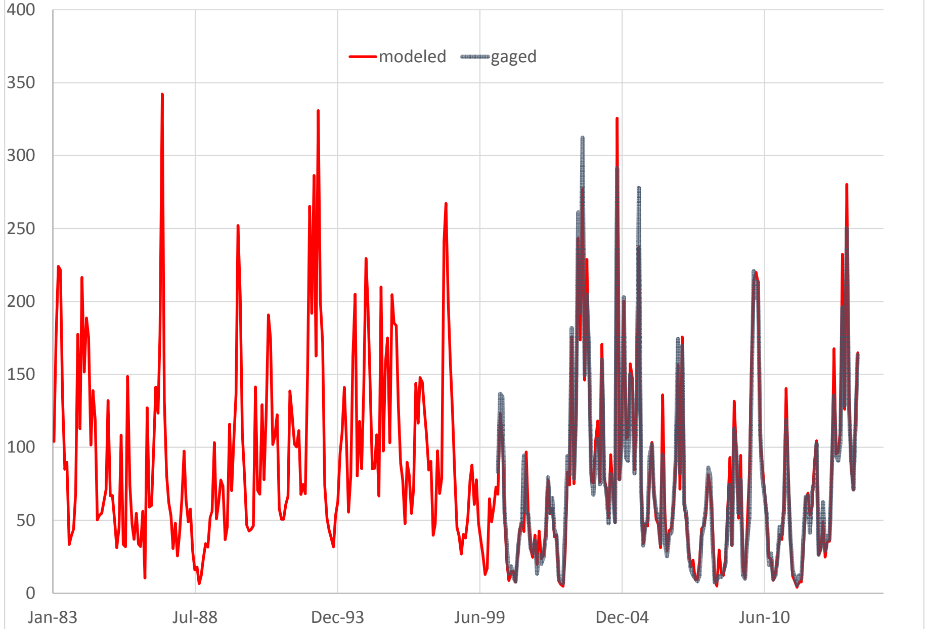
BRD30 (02157510) MIDDLE TYGER RIVER NEAR LYMAN, SC (CFS)
