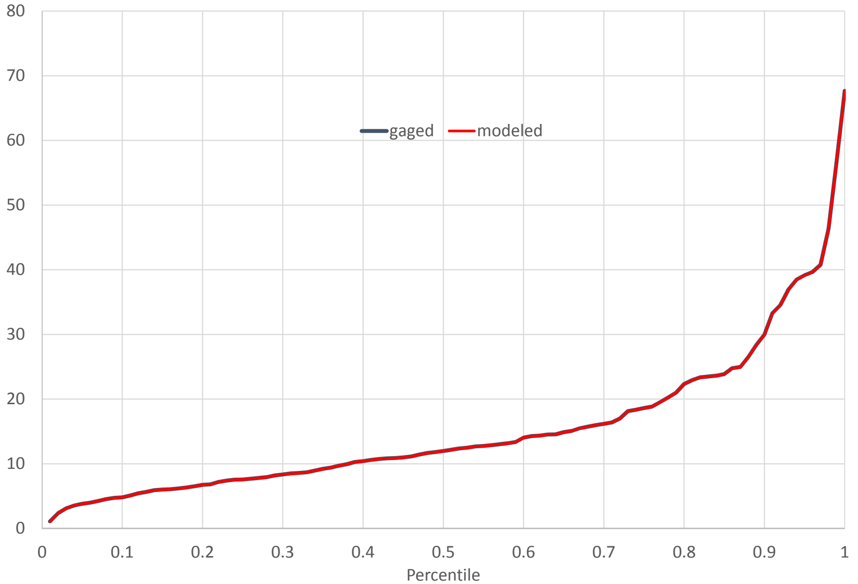
BRD47 (02160381) DURBIN CREEK ABOVE FOUNTAIN INN, SC Monthly Flow Percentiles (CFS)
