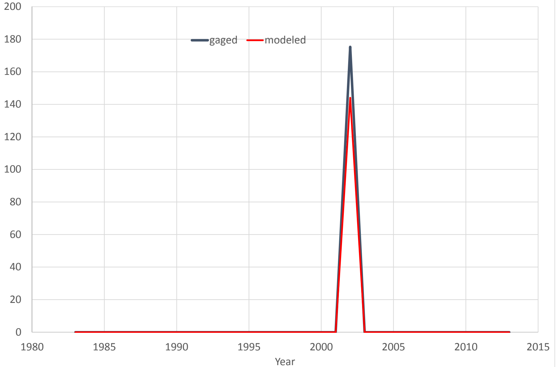
BRD06 (02153680) BROAD R NR HICKORY GROVE, SC Annual 7-day Low Flow (CFS)
