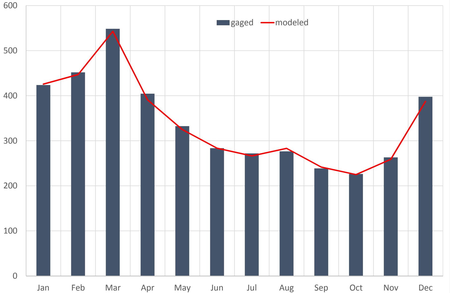
BRD48 (02160390) ENOREE RIVER NEAR WOODRUFF, SC Monthly Mean Flow (CFS)
