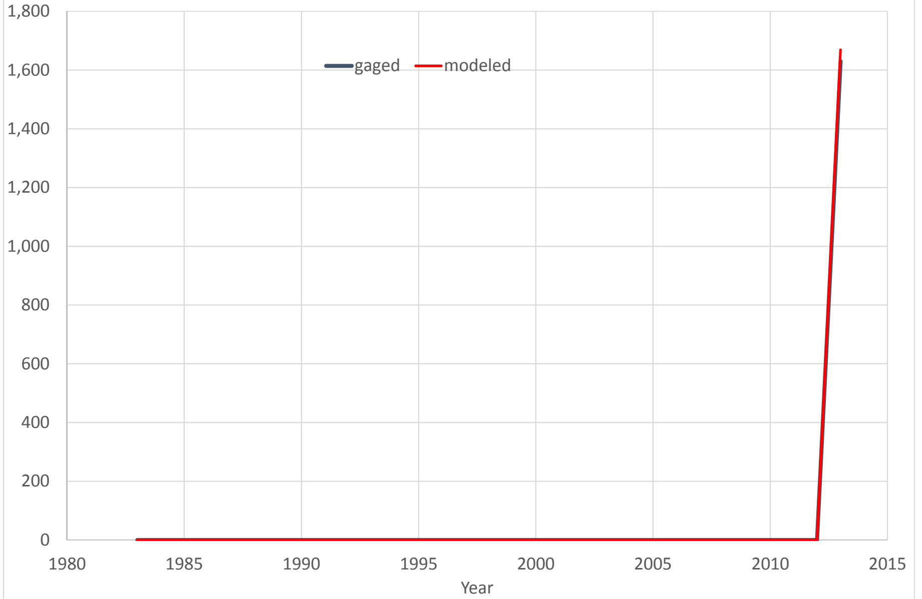
BRD22 (021564493) BROAD RIVER BELOW NEAL SHOALS RES. NR CARLISLE, SC Annual 7-day Low Flow (CFS)
