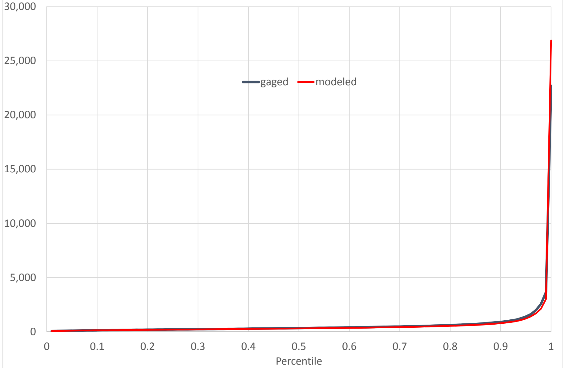
BRD50 (02160700) ENOREE RIVER AT WHITMIRE, SC Daily Flow Percentiles (CFS)
