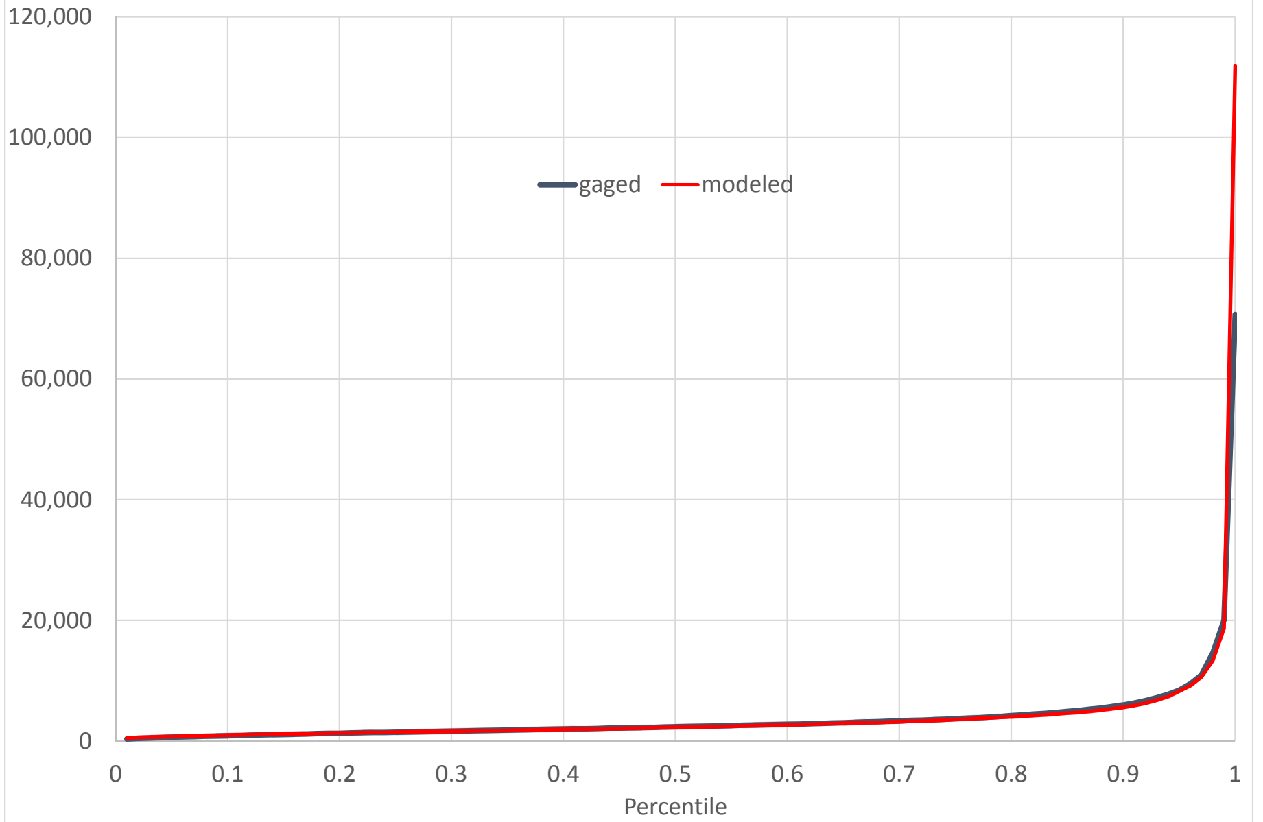
BRD24 (02156500) BROAD RIVER NEAR CARLISLE, SC Daily Flow Percentiles (CFS)
