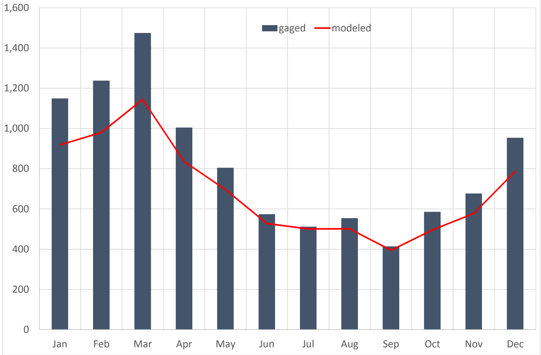
BRD42 (02160105) TYGER RIVER NEAR DELTA, SC Monthly Mean Flow (CFS)
