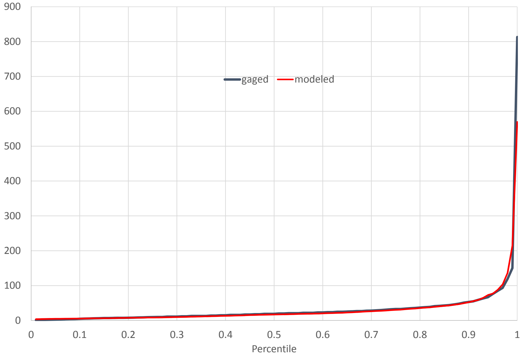
BRD25 (02156999) N. TYGER RIVER BELOW WELLFORD, SC Daily Flow Percentiles (CFS)
