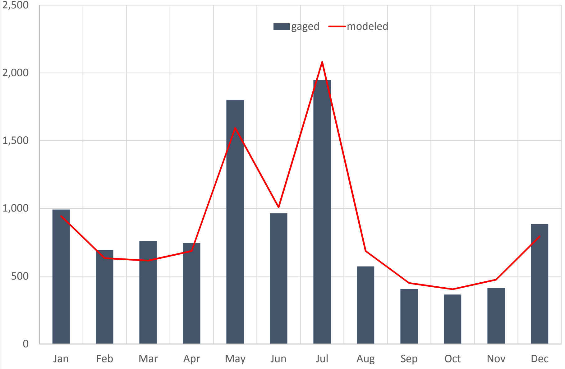
BRD19 (02156370) PACOLET RIVER NEAR SARATT,SC Monthly Mean Flow (CFS)
