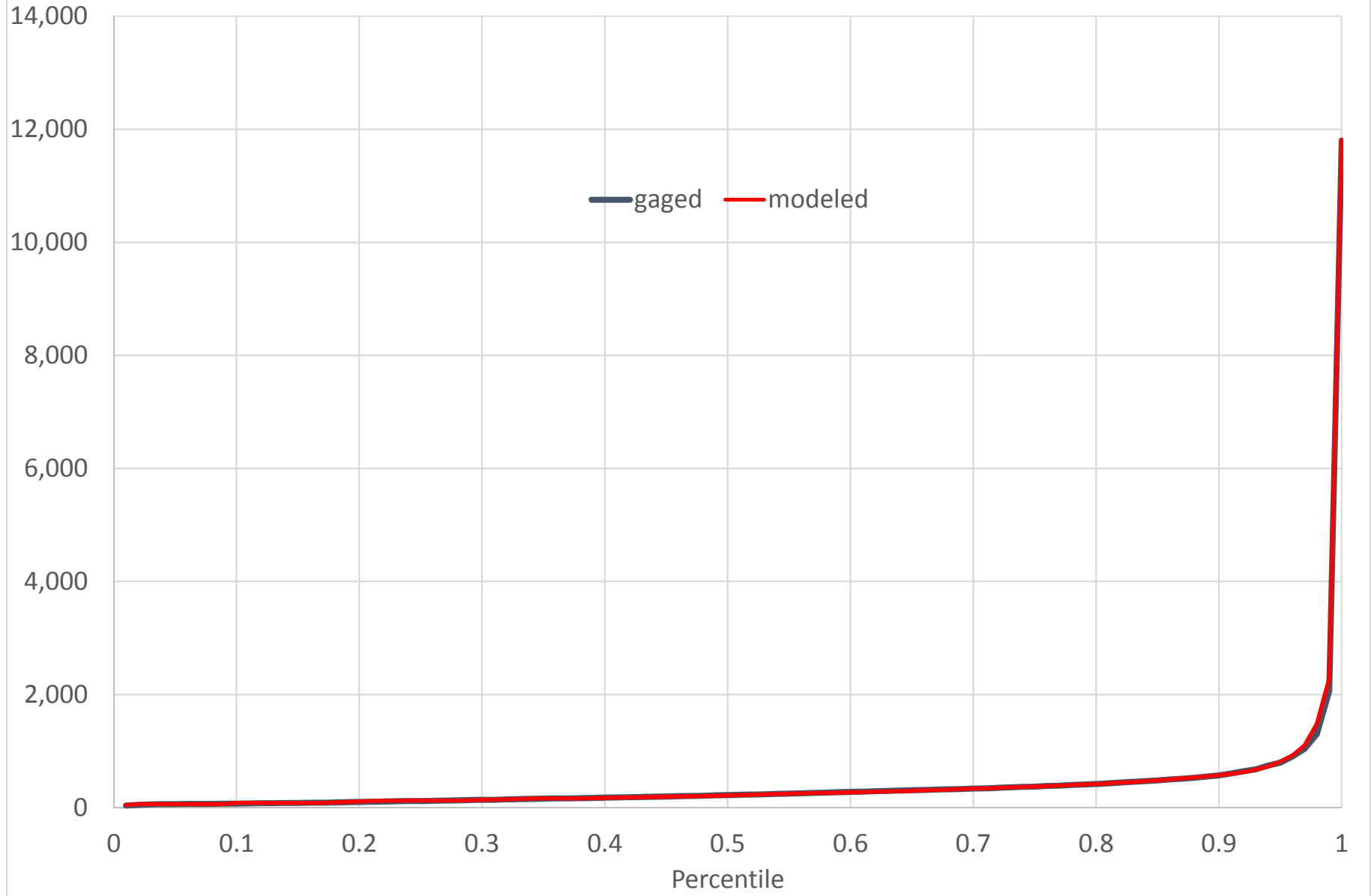
BRD14 (021556525) PACOLET RIVER BELOW LAKE BLALOCK NEAR COWPENS, SC Daily Flow Percentiles (CFS)
