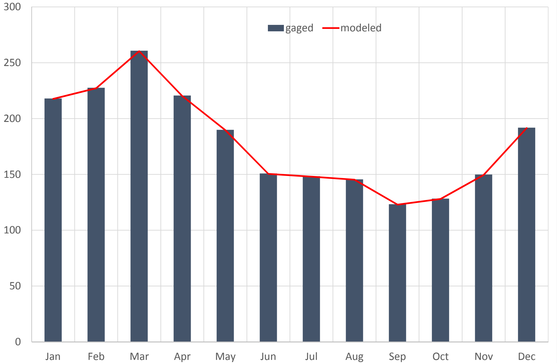
BRD10 (02154500) NORTH PACOLET RIVER AT FINGERVILLE, SC Monthly Mean Flow (CFS)
