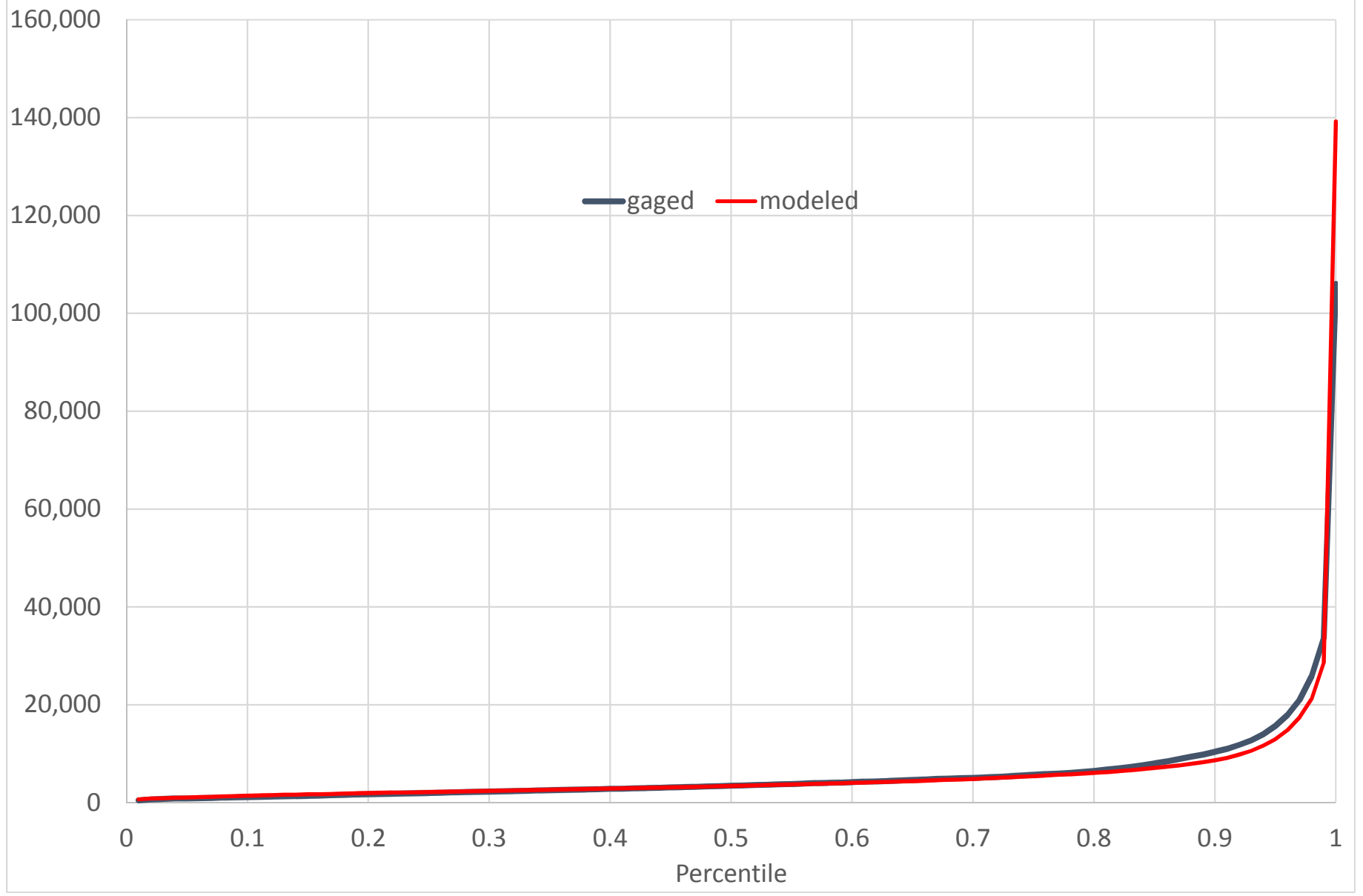
BRD54 (02161000) BROAD RIVER AT ALSTON, SC Daily Flow Percentiles (CFS)
