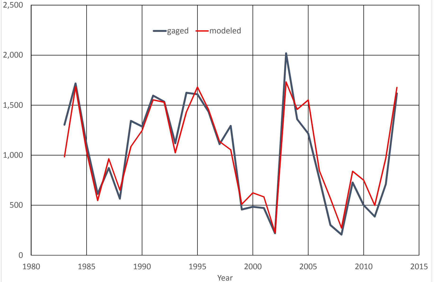
BRD24 (02156500) BROAD RIVER NEAR CARLISLE, SC Annual 7-day Low Flow (CFS)
