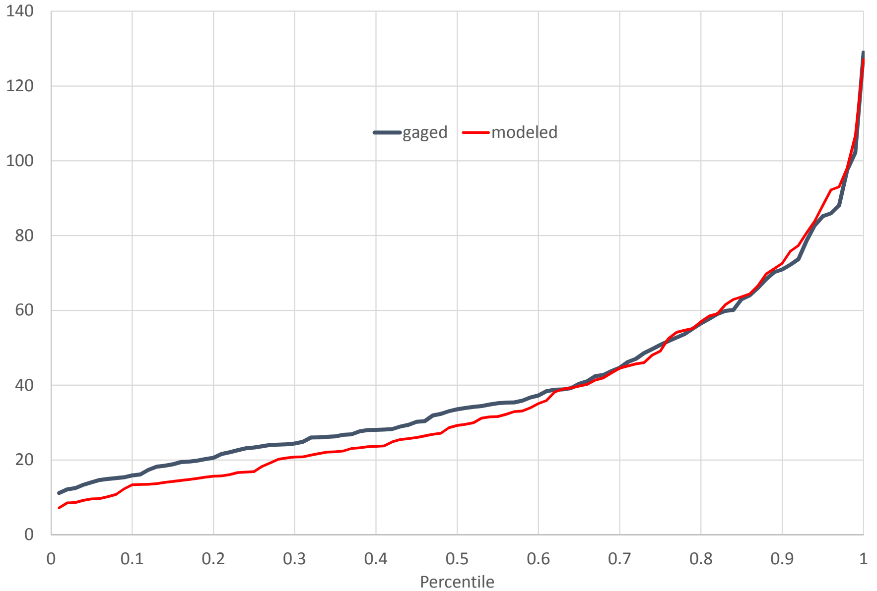
BRD40 (02159810) FAIRFOREST CREEK BELOW SPARTANBURG, S.C. Monthly Flow Percentiles (CFS)
