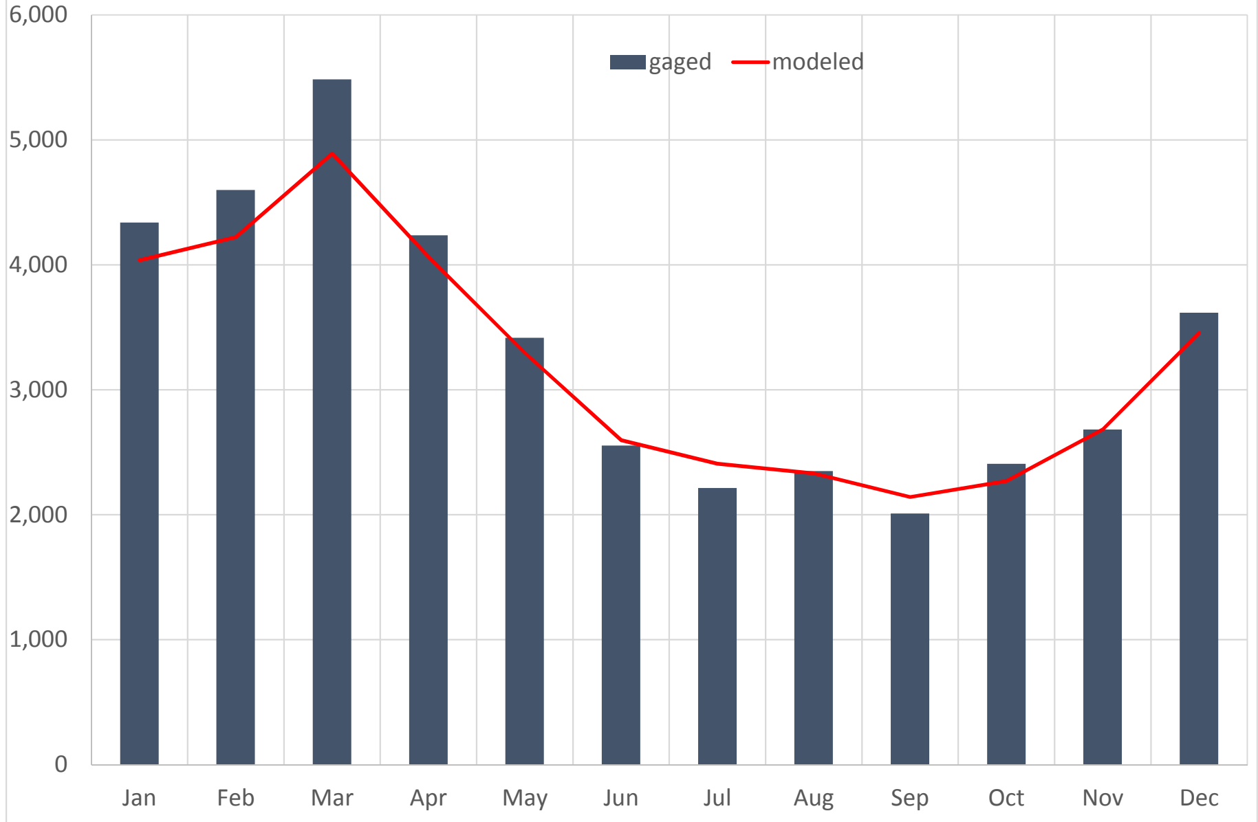
BRD24 (02156500) BROAD RIVER NEAR CARLISLE, SC Monthly Mean Flow (CFS)
