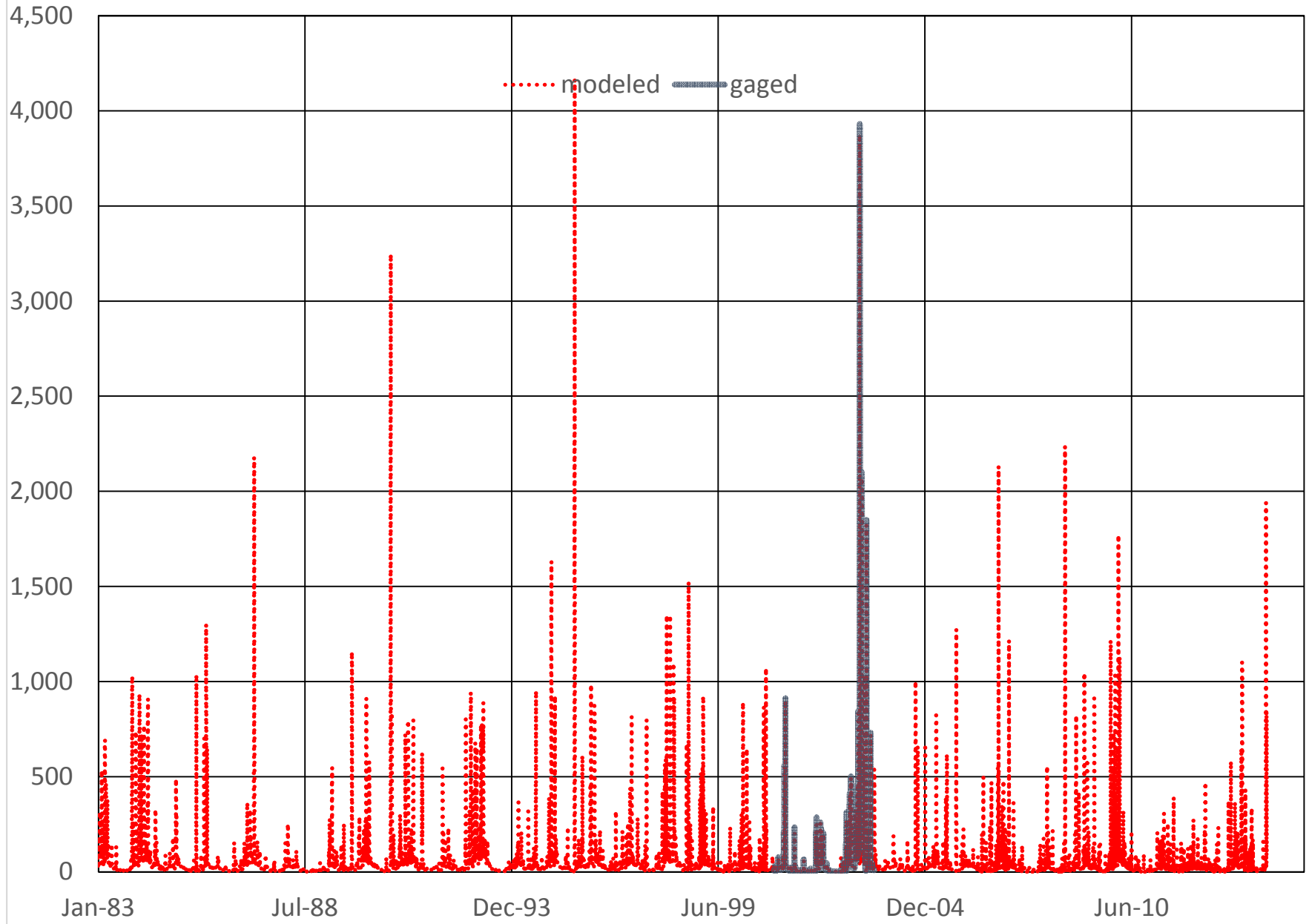
BRD20 (021563931) TURKEY CREEK NEAR LOWRYS, SC (CFS)
