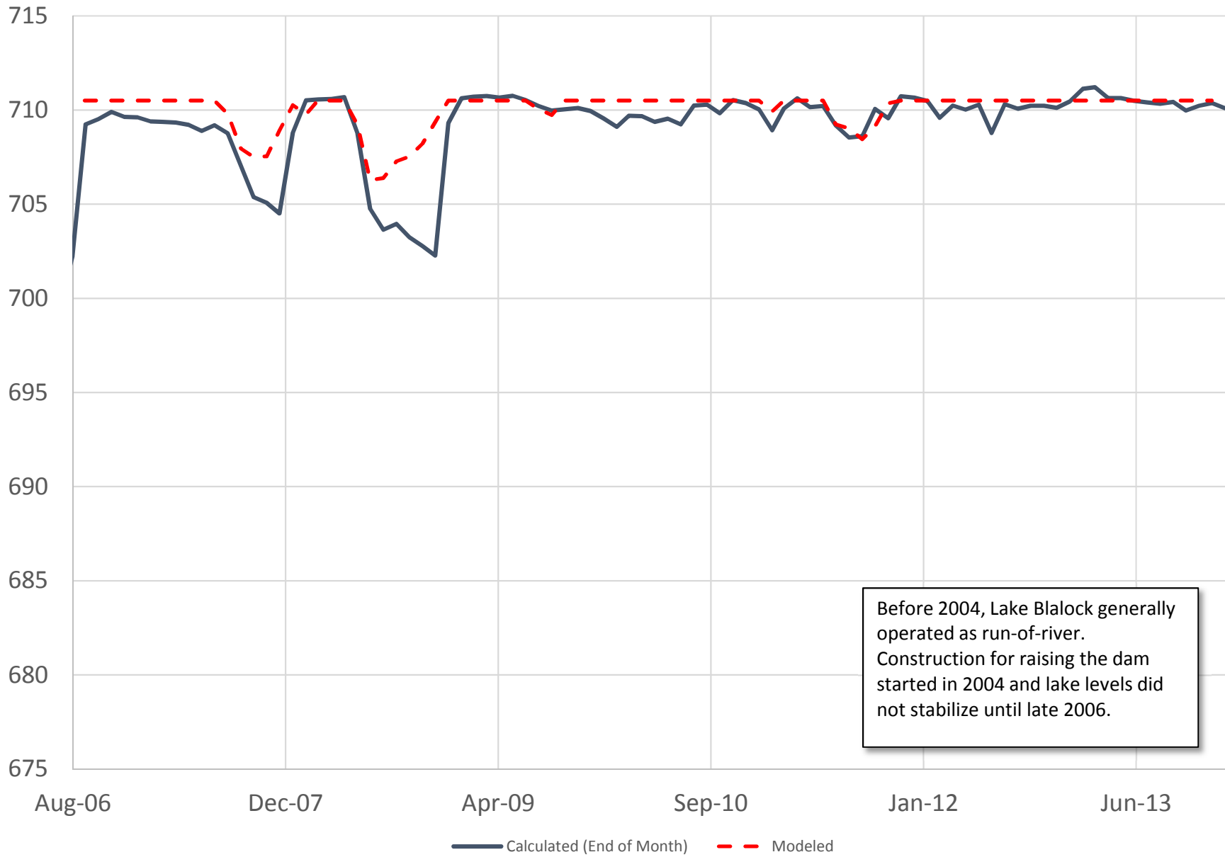
Lake Blalock Elevation (ft)
