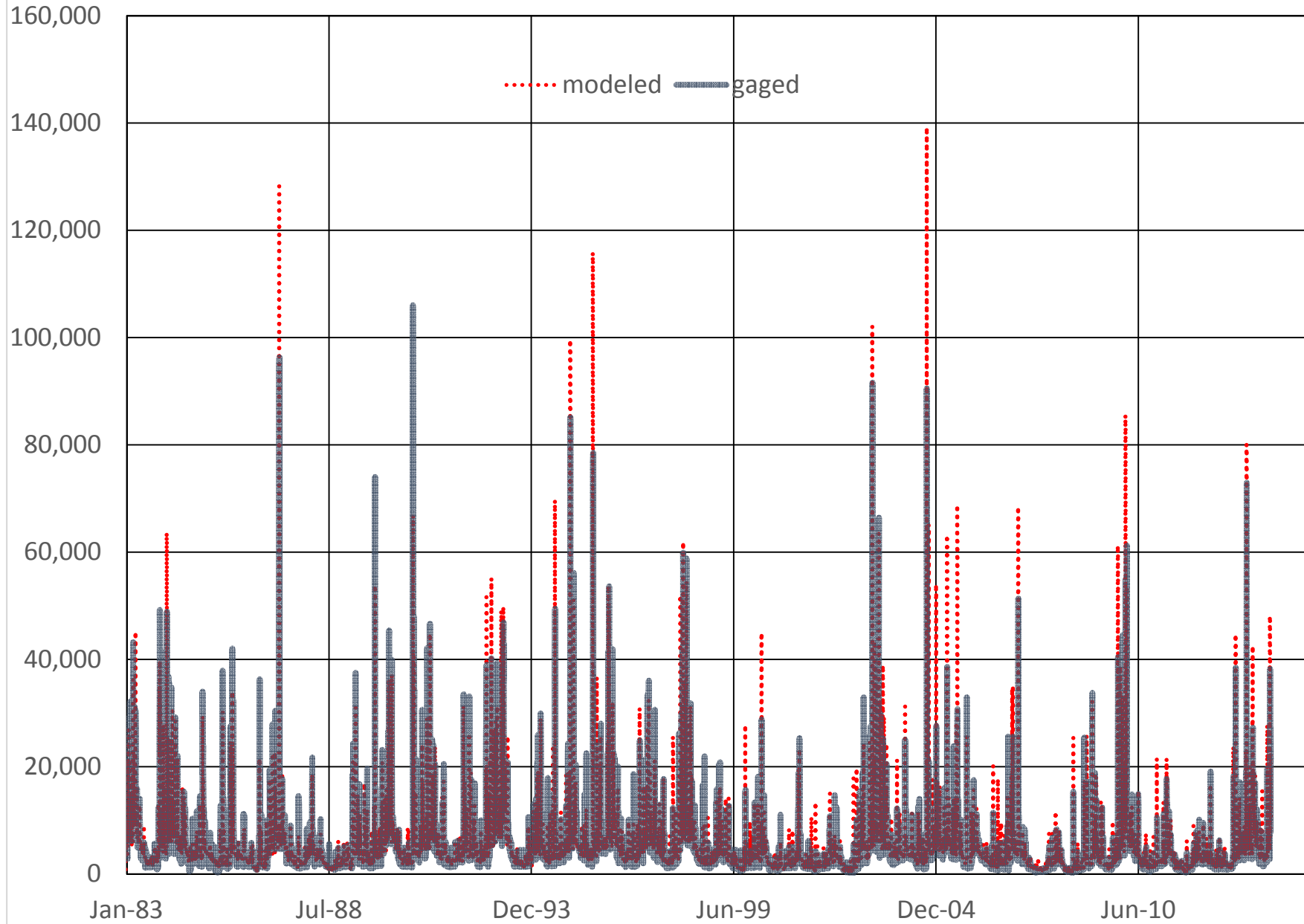
BRD54 (02161000) BROAD RIVER AT ALSTON, SC (CFS)
