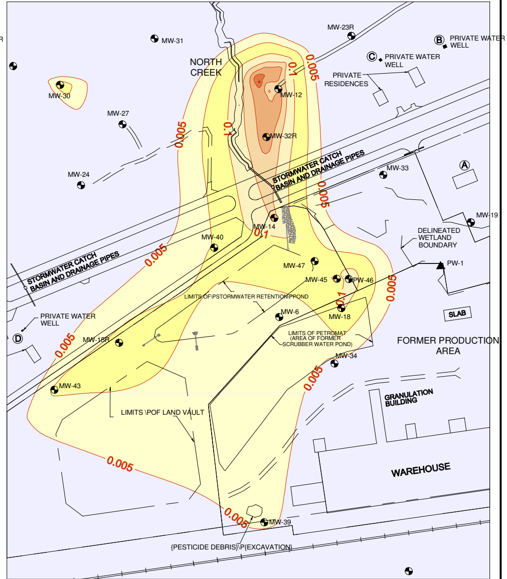
Cadmium Concentrations Greater than 0.005 (mg/L) June 2005
