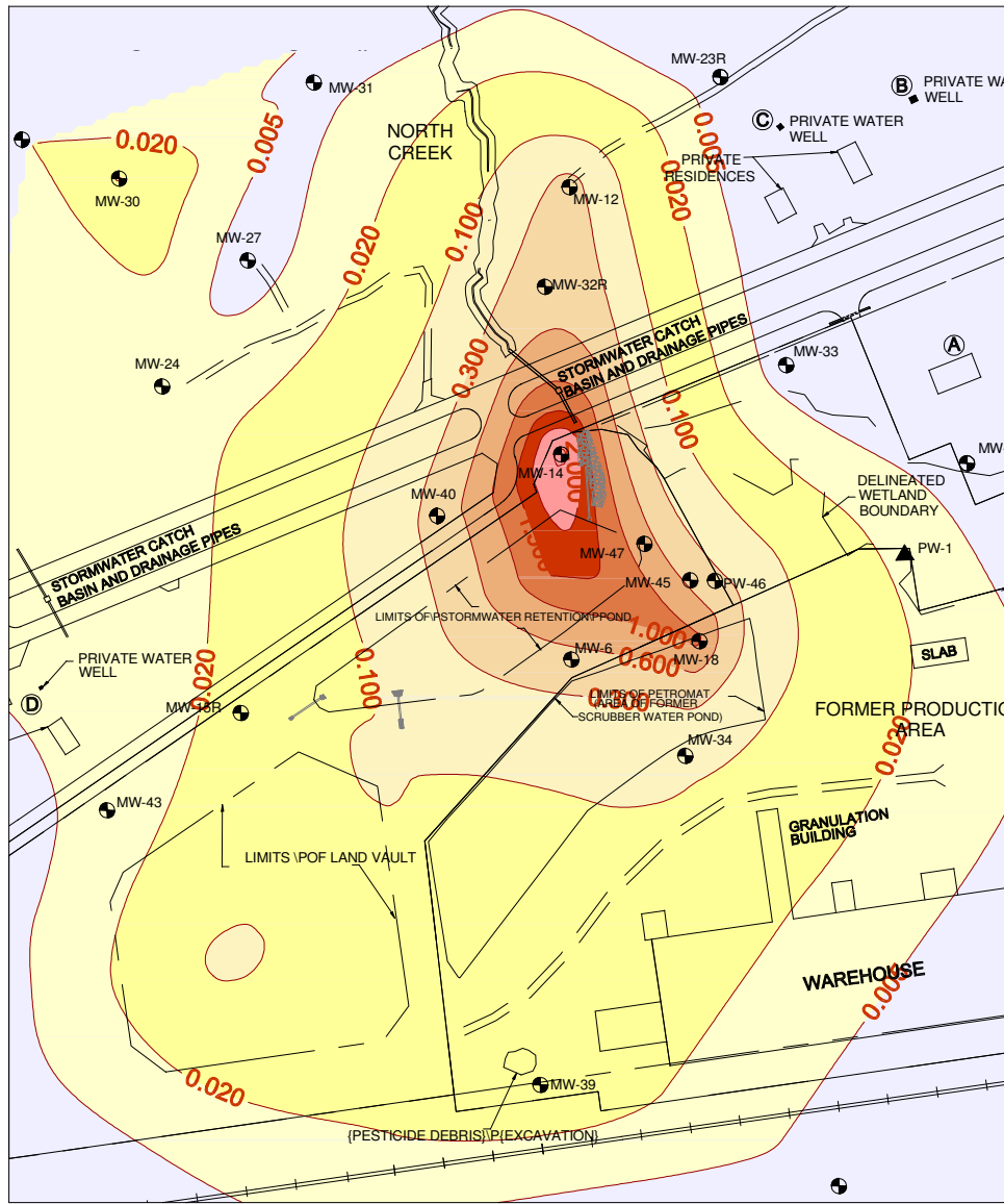
Cadmium Concentrations Greater than 0.005 (mg/L) Initial Conditions (1998)
